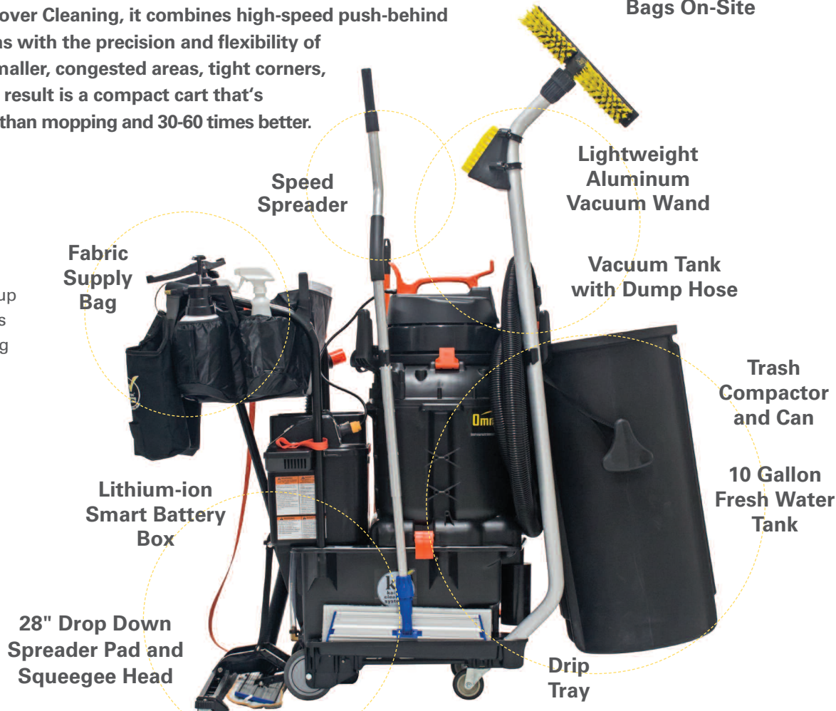
Compactor Wand Vacuum-Shrinks Trash Bags On-Site
